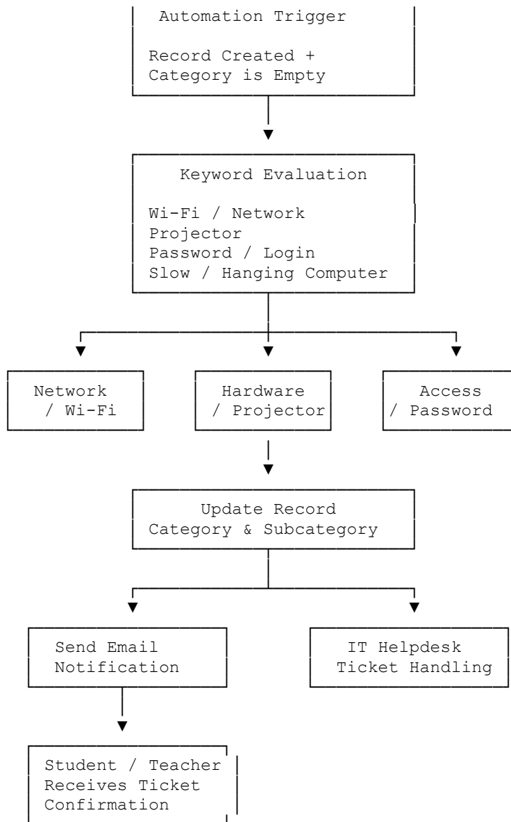
Figure 1: Solution Architecture and Data Flow of Auto Ticket Classification using Flow Designer
